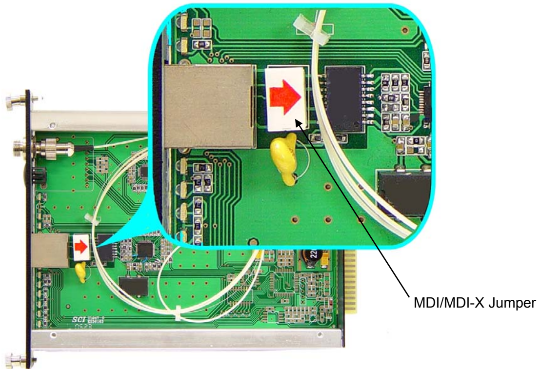
Figure 4.1 Ethernet Module MDI/MDI-X Jumper Location
