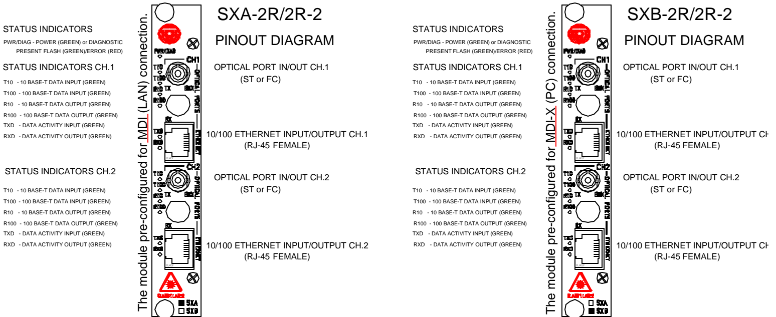
Figure 5.1 10/100 Ethernet Module Front Panel
