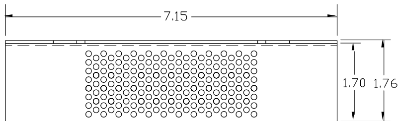
VIEW B
